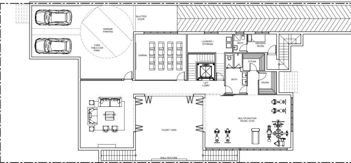
BASEMENT FLOOR
